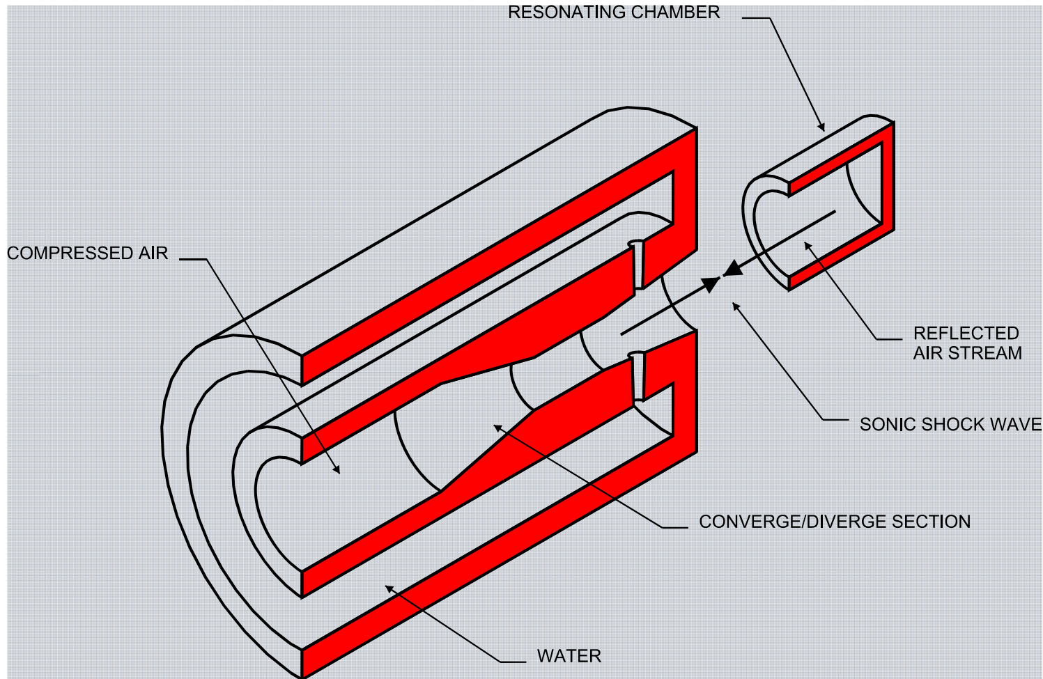
FOGGING NOZZLE CUT-AWAY
